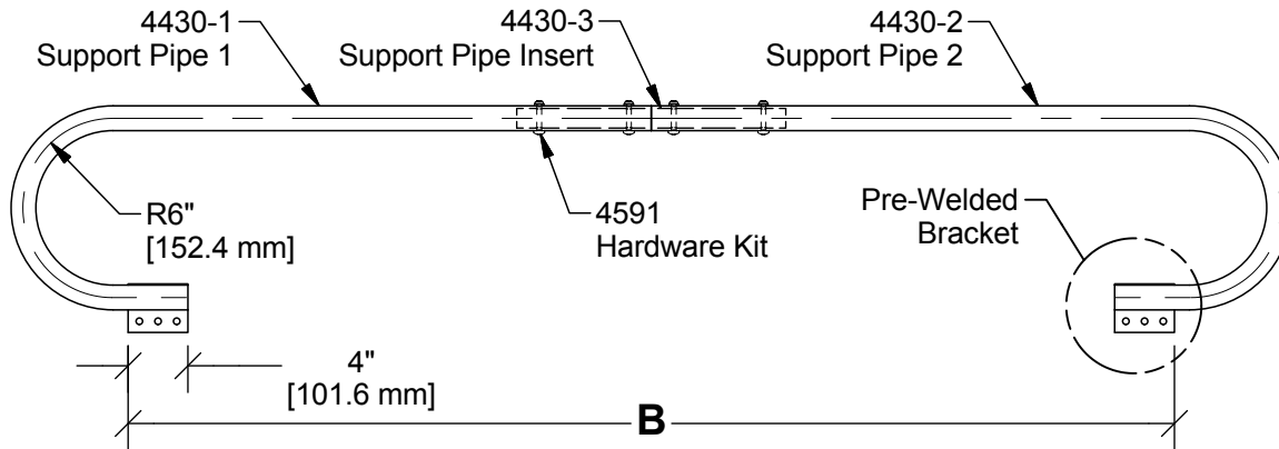
ADJUSTABLE PRESS GUARD PIPE ASSEMBLY
