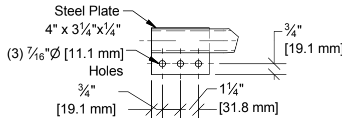
PRE-WELDED BRACKET
